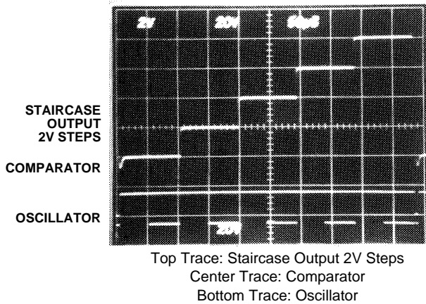
FIGURE 13B. STAIRCASE GENERATOR WAVEFORM
